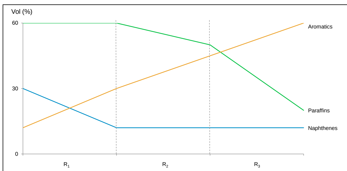
Exhibit 39. Product yields in each reactor
