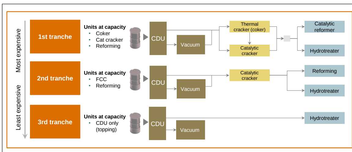
Exhibit 46. Refinery operational tranches
