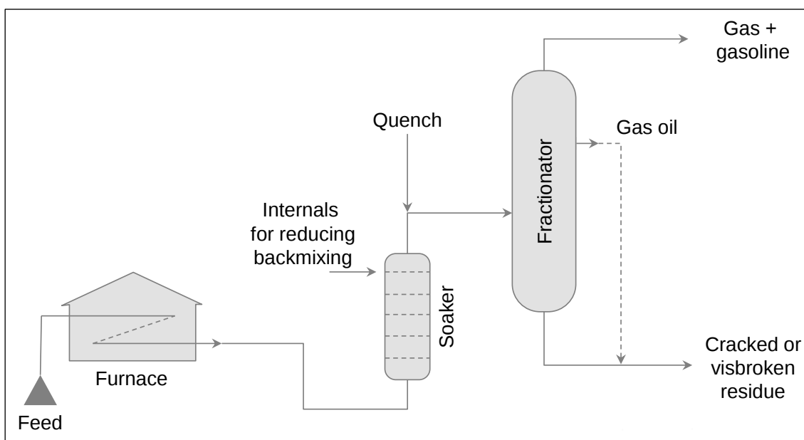
Exhibit 34. Typical visbreaker schematics (soaker type)
