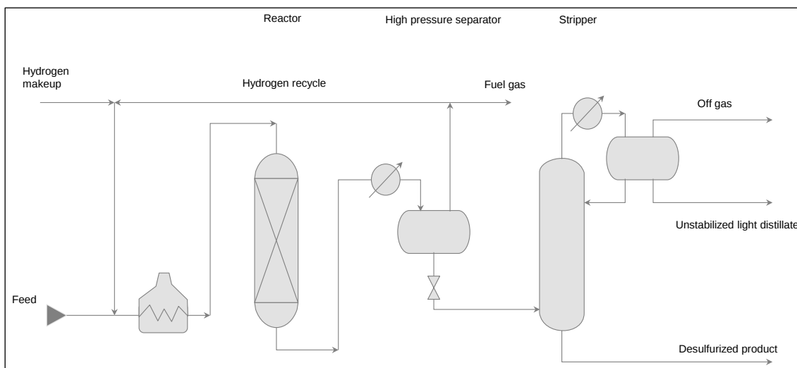
Exhibit 40. Simplified HDS unit schematic
