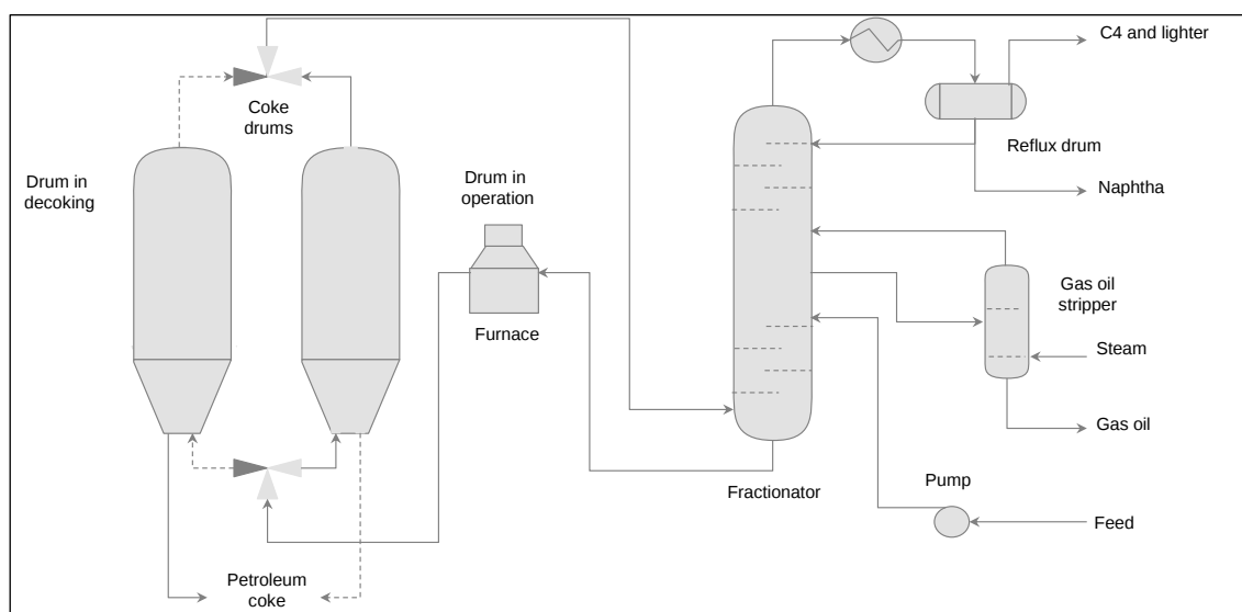
Exhibit 36. Delayed Coker schematic
